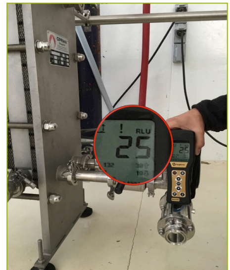
Amount of RLU on Valve from CIP after cleaning with R&T Cleaner
